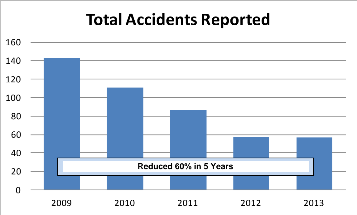
Figure 1-Total Accidents Reported
